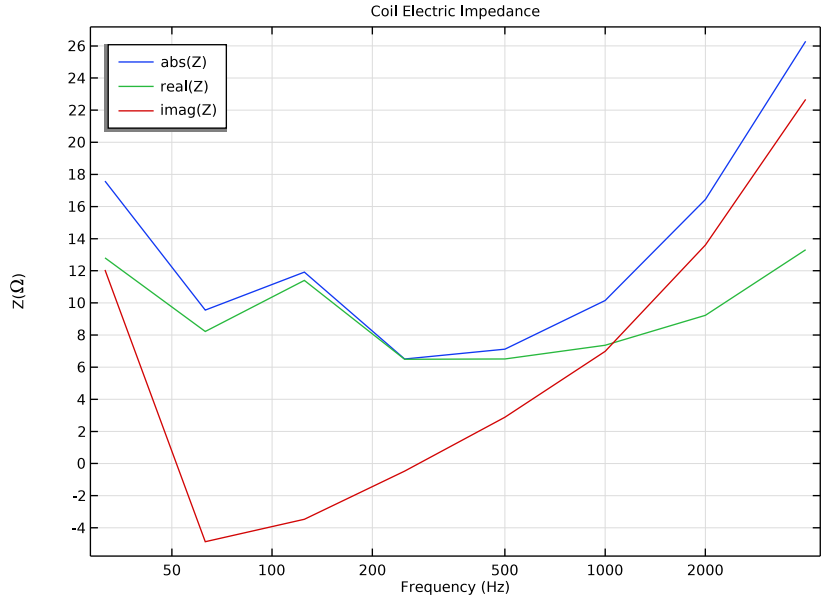
Figure 10: Electric impedance of the voice coil.
