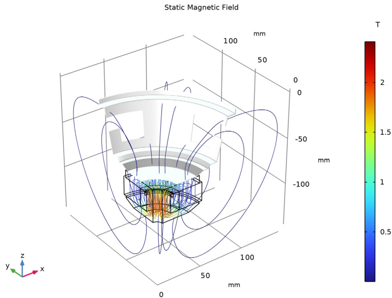
Figure 2: Static magnetic flux density (field lines) of the permanent magnet.
