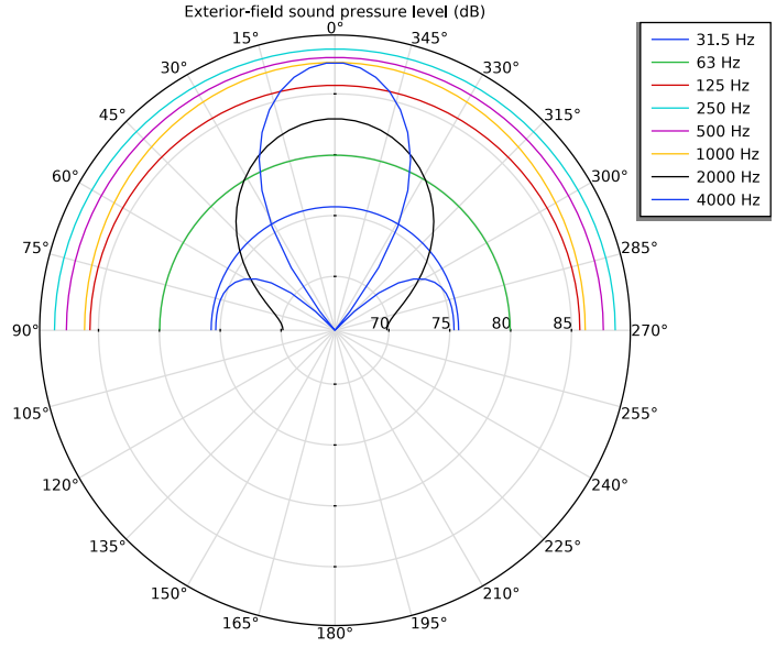
Figure 9: Spatial response in the yz-plane.
