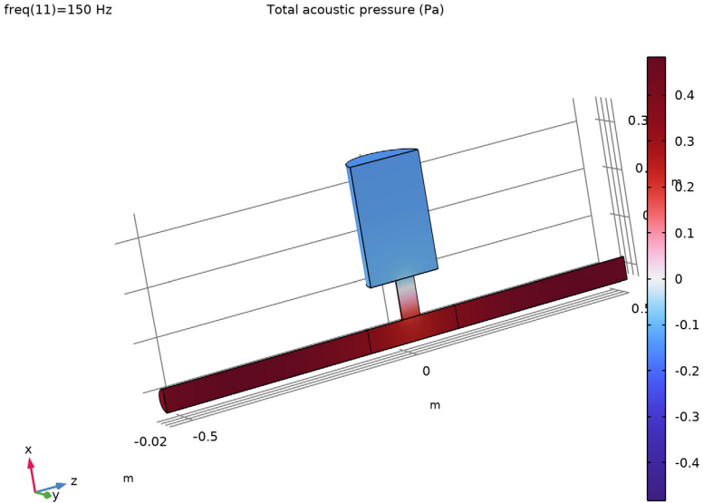
Figure 5: Acoustic pressure in the no flow situation ( Ma = 0 ).
