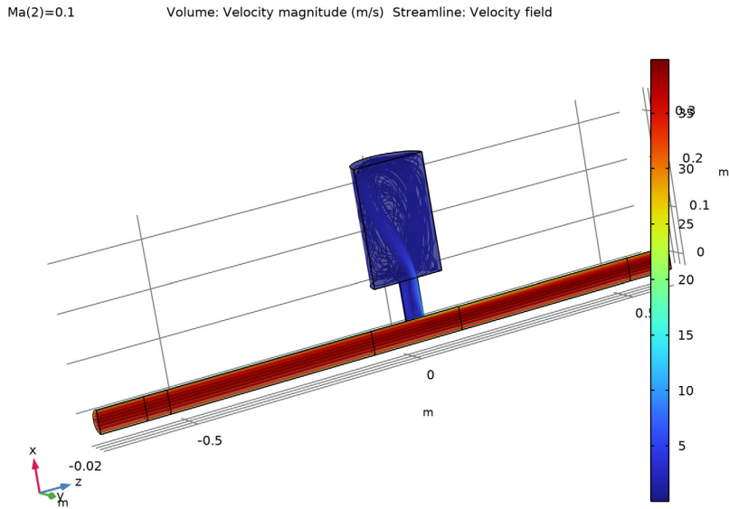
Figure 2: Background mean flow velocity magnitude for Ma = 0.1 .
