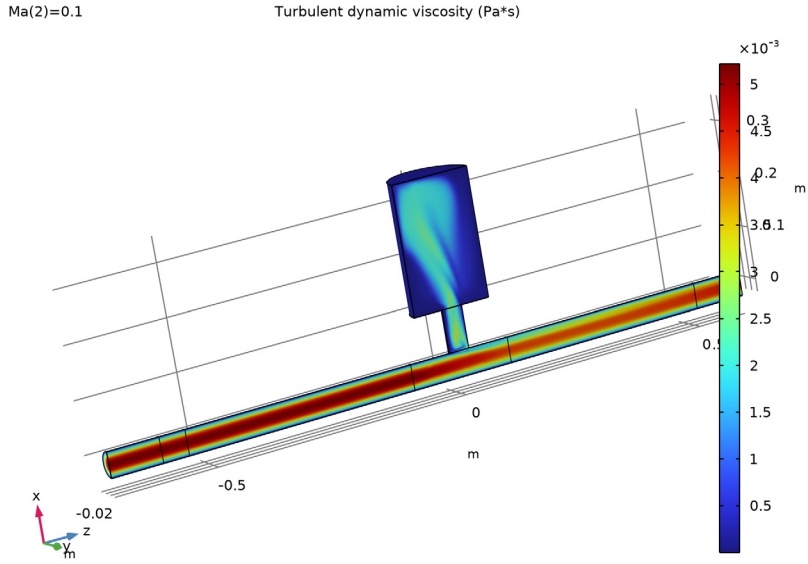
Figure 3: Turbulent viscosity for Ma = 0.1 .
