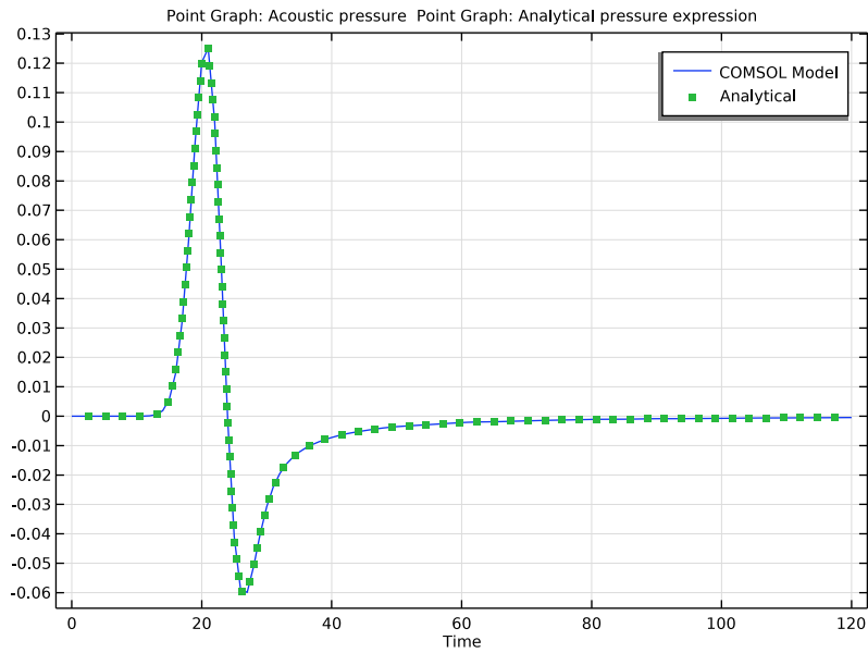
Figure 4: The pressure as a function of time at point (x, y) = (20, 10) . The model solution compared with the analytical solution.
