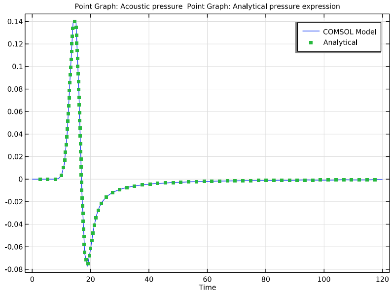
Figure 5: The pressure as a function of time in point (x,y) = (20,30) . The model solution compared with the analytical solution.
