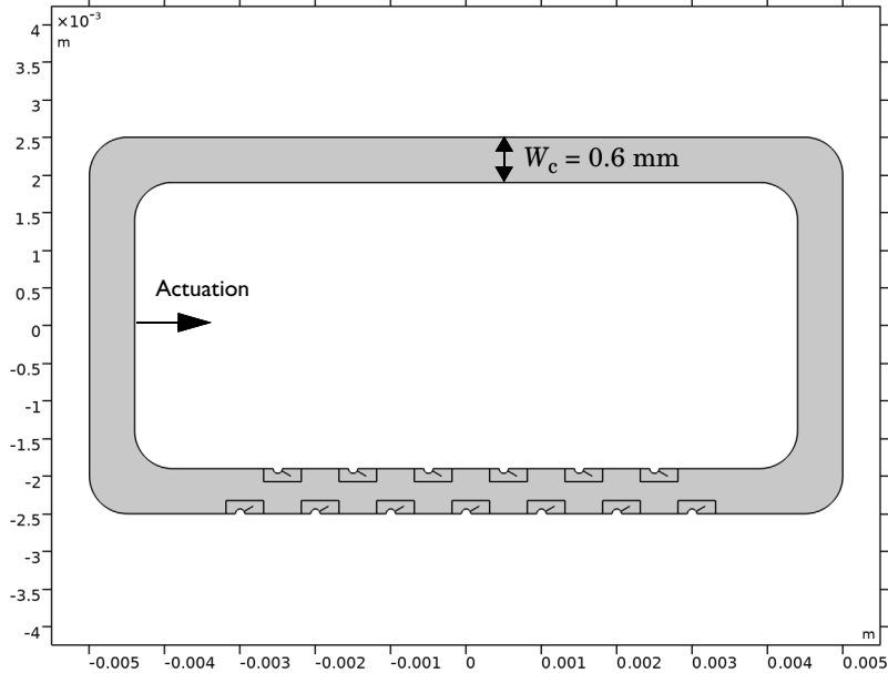
Figure 1: Geometry of the microfluidic pump.
