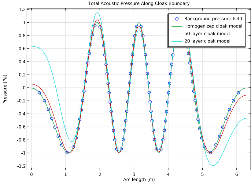
Figure 5: Pressure at the acoustic cloak boundary.
