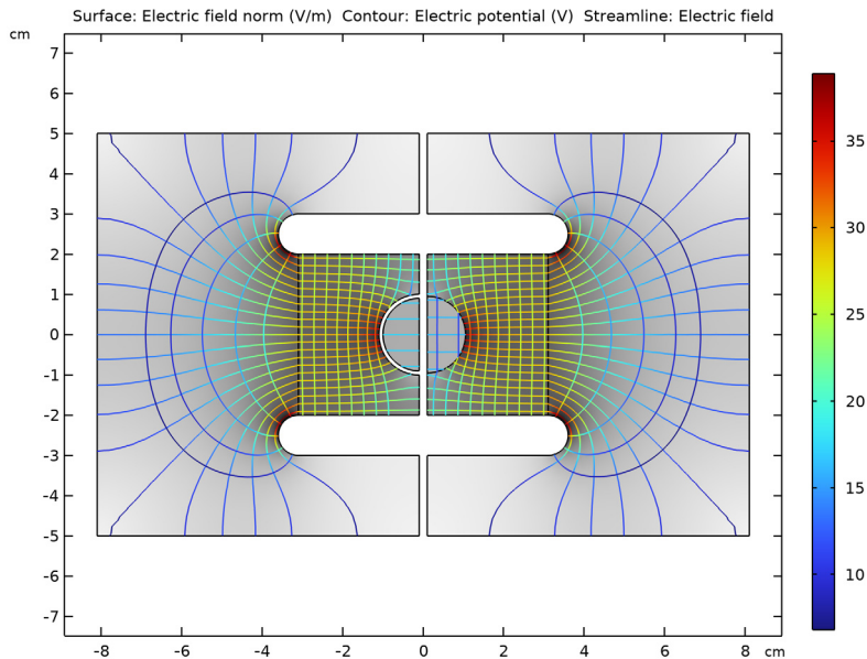
Figure 2: Isolines of the voltage field and streamlines of the electric field are plotted. The lines are colored according to the strength of the electric field, and the background grayscale plot is of the electric field norm. The full fidelity (left) and thin low permittivity gap (right) solutions are almost identical.
