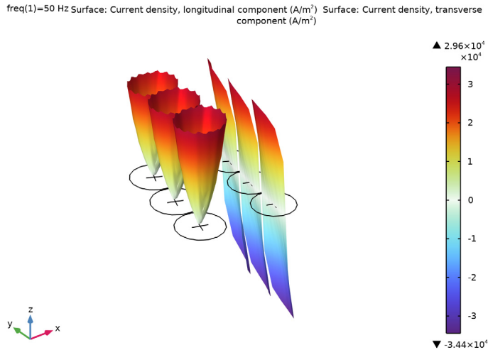
Figure 7: The transverse currents form eddies in the cross section of the wire (the cones), the longitudinal currents flow back and forth and are zero on average (the gradients). An animated version is available as reference [9].
