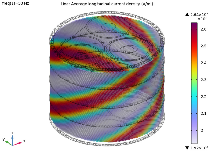
Figure 9: The average longitudinal current density in the armor, before applying the compensation term.
