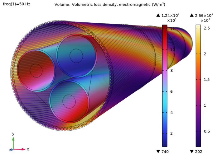
Figure 8: The volumetric loss density in the armor and screens, for the case where a first-order temperature correction has been applied.
