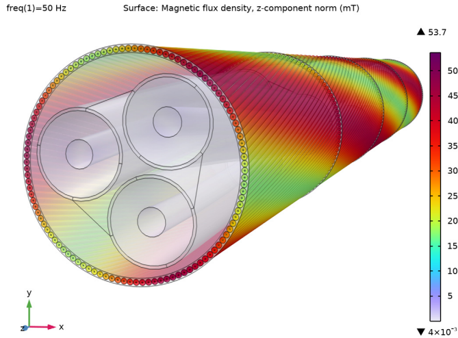
Figure 5: The norm of the longitudinal magnetic flux density component.
