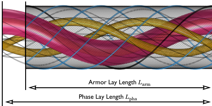
Figure 2: The cable's armor lay length and phase lay length (image scaled by a factor of 5 in the longitudinal direction). The lay length is the distance required for the helices to complete a full revolution.
