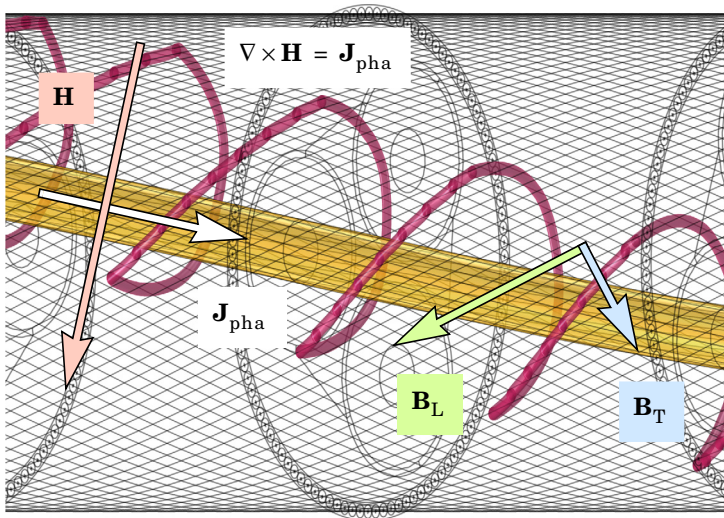
Figure 6: The magnetic field \mathbf{H} encircles the phase conductor. Having arrived at the armor, the flux can choose between a longitudinal direction \mathbf{B}_L , or a transverse one \mathbf{B}_T .
