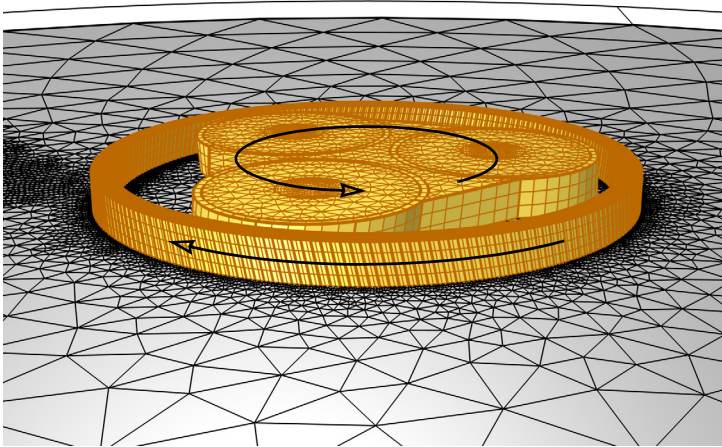
Figure 4: The mesh in the armor rotates clockwise, while the remaining mesh rotates counterclockwise. The source periodicity plane is at the bottom, and the destination is at the top.
