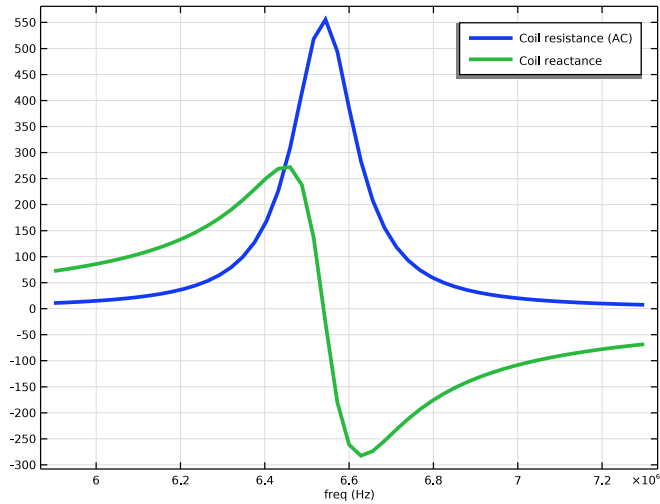
Figure 3: The feed impedance (resistance and reactance) is shown. Note the transition from inductive (positive) to capacitive (negative) reactance at the resonance frequency.
