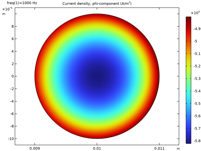
Figure 7: The real part of the induced currents in the secondary coil for the closed circuit case.
