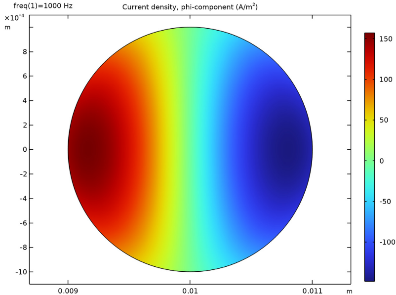
Figure 6: The real part of the induced currents in the primary coil for the open circuit case. The net current flow over the cross section is zero, this is true independently of phase.
