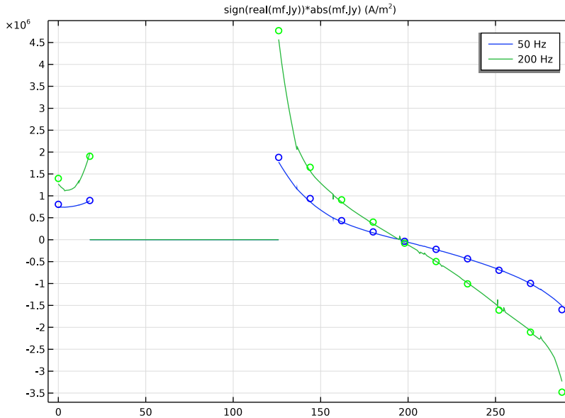
Figure 5: y -components of the induced current densities, J_y ( A/m^2 ) for 0 \leq x \leq 288 mm at y = 72 mm, z = 19 mm for 50 Hz and 200 Hz. The solid lines are simulation results while the circles are the corresponding measured data from Ref. 1.
