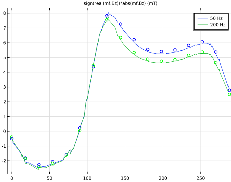
Figure 4: z -component of the flux density, B_z (mT), at 0 \leq x \leq 288 mm, y = 72 mm, and z = 34 mm for 50 Hz and 200 Hz. The solid lines are simulation results while the circles are the corresponding measured data from Ref. 1.
