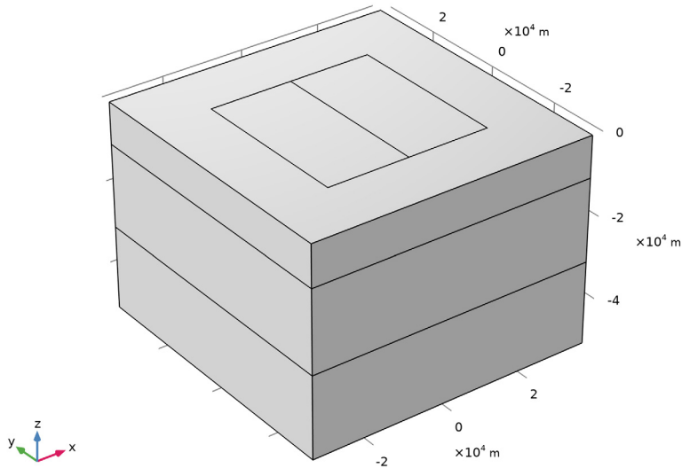
Figure 1: A 70 by 70 km piece of Earth's crust, consisting of three layers of different conductivities. From top to bottom, the conductivities are 10, 100, and 0.1 \Omega\text{m} . The upper layer has two rectangular inserts of conductivities 1 and 100 \Omega\text{m} .
