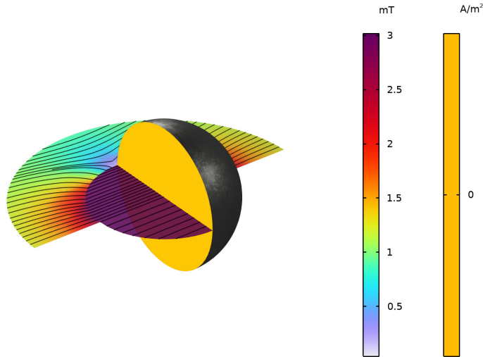
Figure 2: Cross section of the iron sphere in a static magnetic field. The magnetic flux shows the distortion of the background magnetic field caused by the permeable iron sphere. There are no induced currents in this model.
