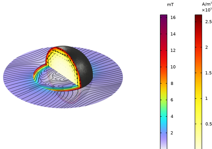
Figure 4: Cross section of the iron sphere in a time varying background magnetic field oscillating at 20 kHz.
