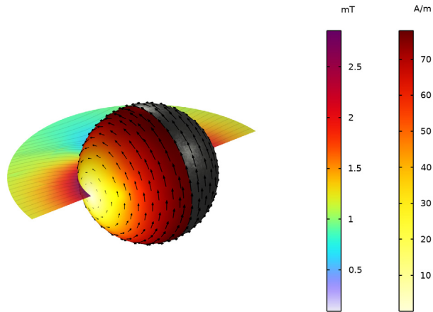
Figure 5: Surface of the iron sphere in a time varying background magnetic field oscillating at 13.56 MHz.
