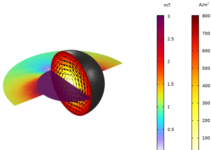
Figure 3: Cross section of the iron sphere in a time varying background magnetic field oscillating at 60 Hz.
