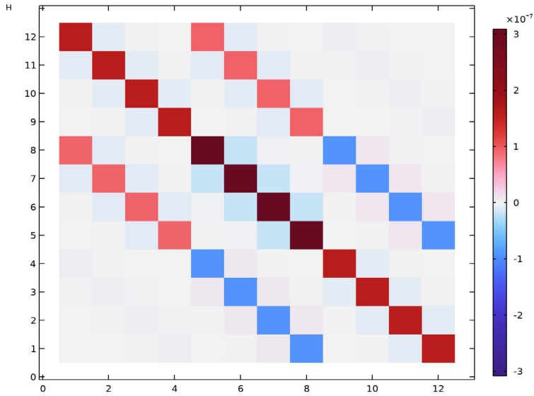
Figure 3: Visualization of the inductance matrix of PCB coils, stationary solution.
