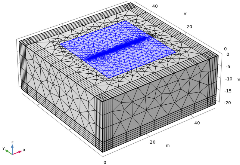
Figure 2: Refined mesh around the electrodes and swept mesh in infinite element regions.
