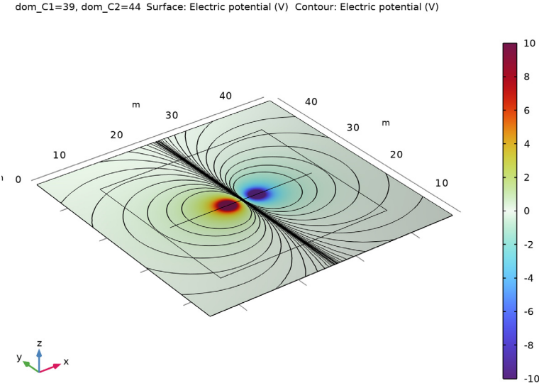
Figure 3: Electric potential around the active electrode pair.
