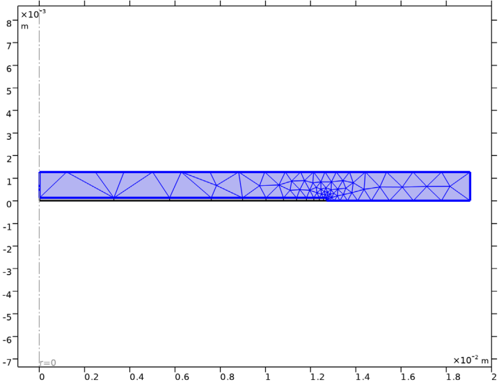
Figure 2: Model mesh.
