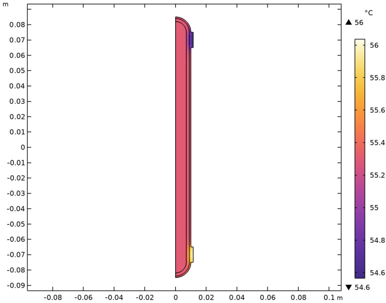
Figure 10: Temperature of heat pipe with saturated wick.
