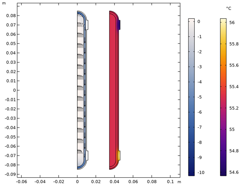
Figure 11: Fluid velocities— \lg(|\mathbf{u}| / \text{m}\cdot\text{s}^{-1}) and temperature in the heat pipe running at the design point.
