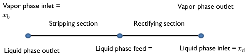
Figure 13: One-dimensional model geometry including the boundary conditions for the mole fraction of ethanol in each phase.
