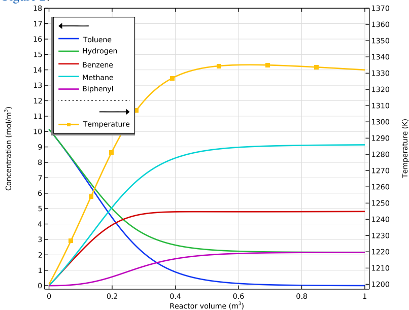
Figure 2: Species concentrations (mol) and temperature (K) as function of reactor volume ( m^3 ) for a tubular reactor design.
