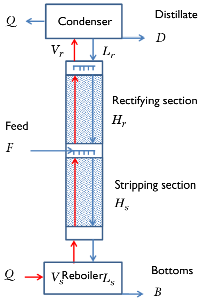
Figure 12: Packed distillation column schematic.
