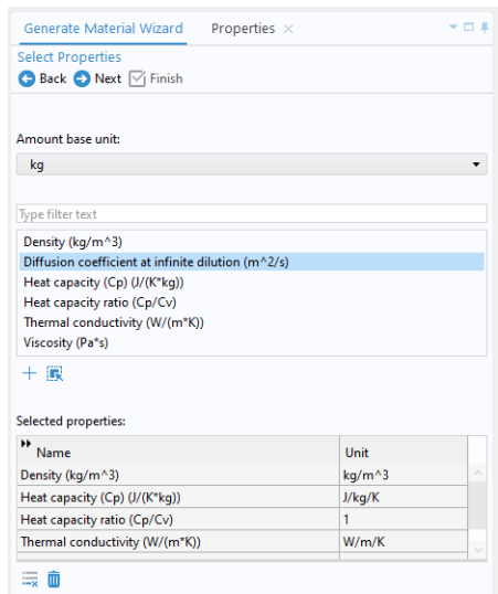
Figure 10-23: Generate Material Wizard; Select Properties pane with Diffusion coefficient at infinite dilution added.
