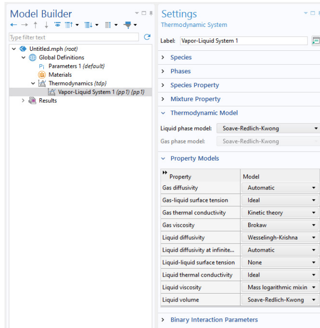
Figure 10-6: Thermodynamic System Settings.
