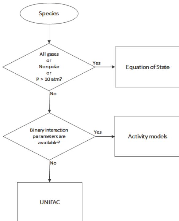
Figure 10-37: Decision tree to select thermodynamics model.
