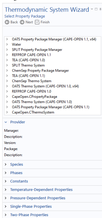
Figure 10-9: Available external thermodynamic systems. Use the Thermodynamic System Wizard to browse the contents of the installed external thermodynamic systems on your system. The example shows the packages shipped with the COCO provider.
