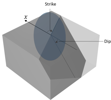
Figure 1: Strike and dip directions.
