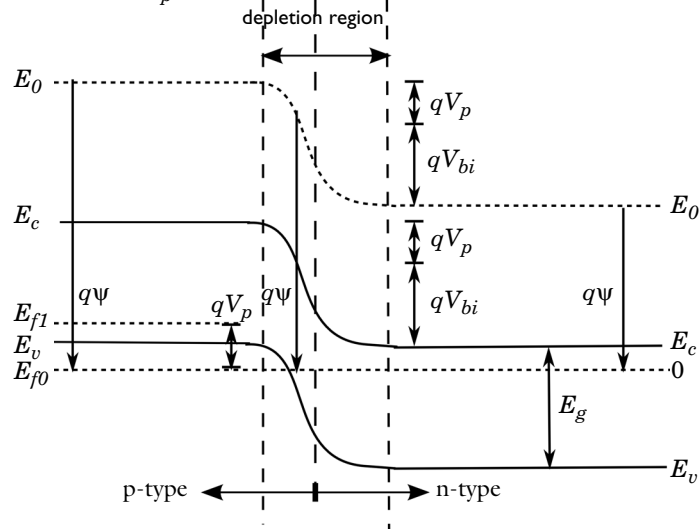
Figure 3-7: Diagram showing the variation in the band structure in a p-n diode. The horizontal axis represents position in the device and the vertical axis indicates energy. The vacuum level E_0 , the bottom of the conduction band E_c , and the top of the valence band E_v , are shown. Top: The band structure when there is no applied potential. A built-in potential, V_{bi} , develops across the junction as a result of the space charge layers associated with the depletion region. The Fermi energy E_{f0} , is constant throughout the device. Bottom: A potential V_p is applied to the n-type side of the junction, resulting in a reverse bias. Away from the junction, where the material is close to equilibrium, a second Fermi level, E_{f1} , can be defined in the p-type region, shifted by the applied potential.
