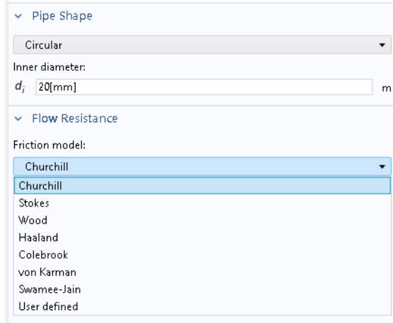
Figure 11: Select a shape and different predefined friction models in the Pipe Properties node.
