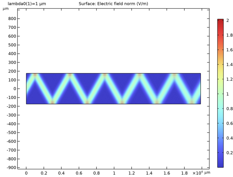
Figure 2: Simulation result showing the electric field norm. The plot is scaled ten times in the y direction.
