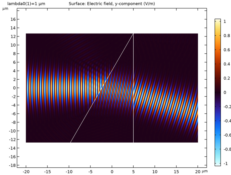
Figure 3: Dominant electric field component of a p-polarized Gaussian beam propagating from left to right through a right angle triangular optical prism.
