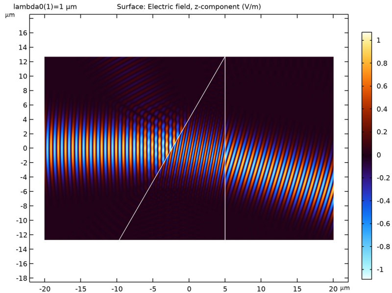
Figure 2: Electric field component of an s-polarized Gaussian beam propagating from left to right through a right-angled triangular optical prism.
