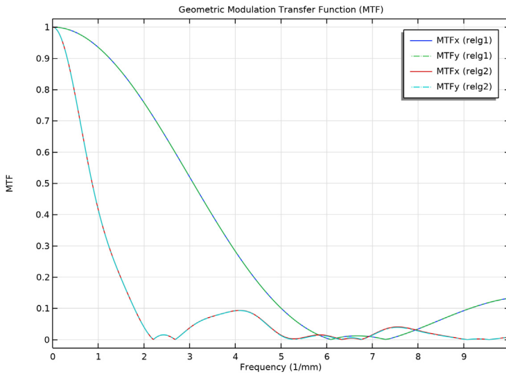
Figure 4: Geometric modulation transfer function (MTF).
