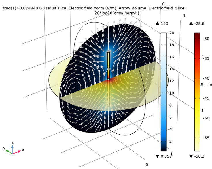
Figure 2: A slice plot of the electric and magnetic field magnitude around the antenna.
