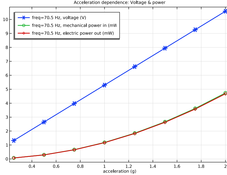
Figure 4: DC voltage and mechanical/electric power output versus the magnitude of the mechanical acceleration at a fixed frequency of 70.5 Hz with a load impedance of 12 k \Omega .
