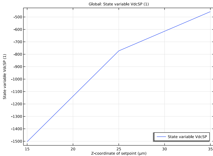
Figure 3: VdcSP versus z_{sp} = 35, 25 , or 15 \mu m , without helium gas flowing.
