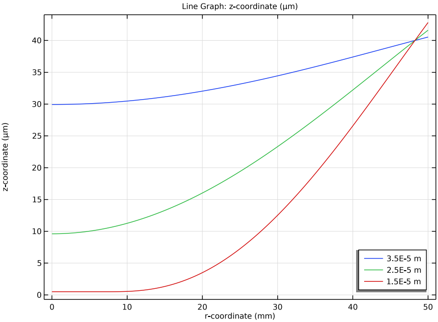
Figure 2: Wafer profile when zsp is set to 35, 25, and 15 \mu\text{m} without helium gas flowing. As expected. The structural displacement is maximal at the center of the geometry. For zsp = 15 \mu\text{m} , the center of the wafer is in contact with the e-chuck.
