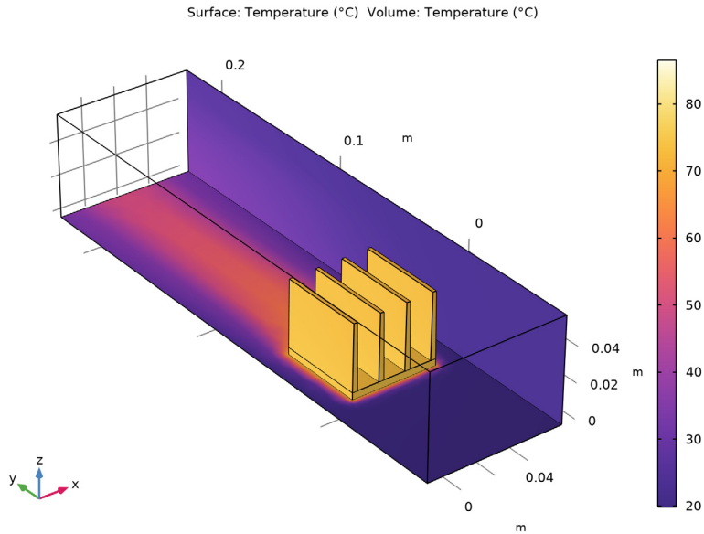
Figure 5: The surface plot shows the temperature field on the channel walls and the heat sink surface.
