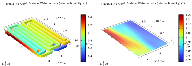
Figure 5: Left: Relative humidity in the channels. Right: Water activity in the membrane.
