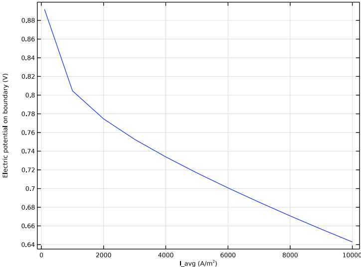
Figure 2: Polarization plot.
