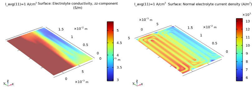
Figure 6: Left: Electrolyte conductivity in the membrane. Right: Electrolyte current density in the z direction.
