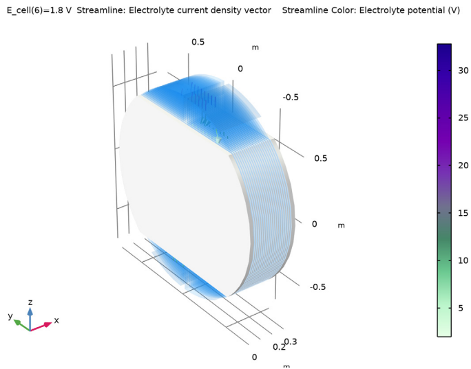
Figure 5: Current streamlines in the inlet and outlet channels and manifolds.
