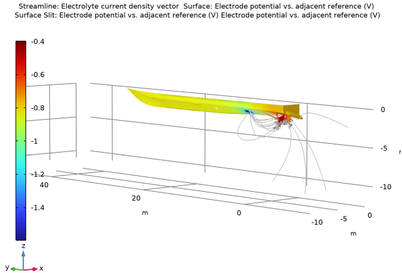
Figure 7: A surface plot of the hull potential for the case of an uncoated propeller.
