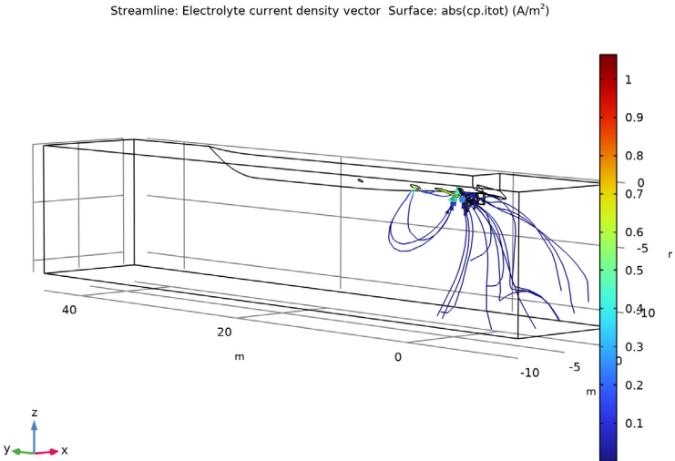
Figure 6: A surface plot of the total current density for the case with a coated propeller.
