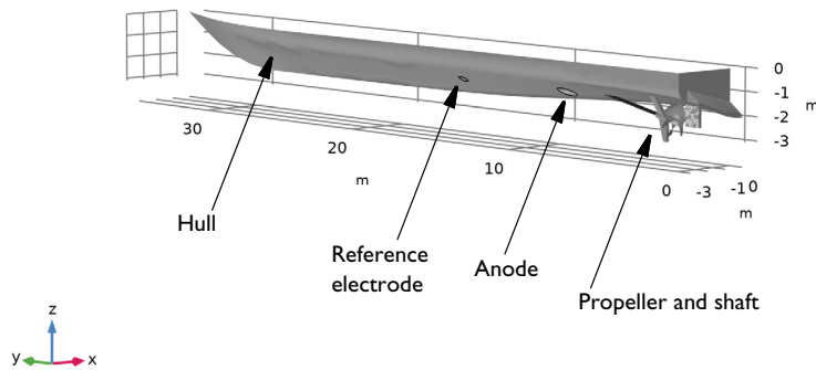
Figure 1: The geometry of the ship hull surface, which is exposed to the sea water.
