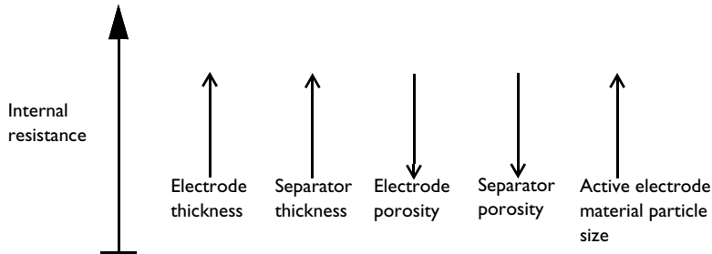
Figure 1: Selection of design parameters in a cell and their relation to increased internal resistance. Upward pointing arrows indicate increase, downward pointing decrease. For example, the internal resistance increases with decreased porosity and increased particle size.
