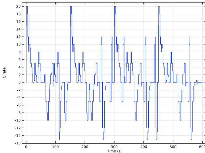
Figure 2: Drive cycle, defined as C-rate versus time.
