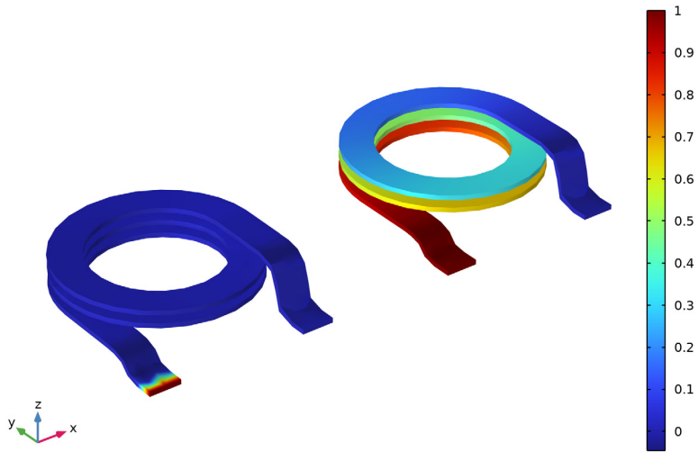
Figure 2: Comparison of the electric potential distribution on the coil between ungauged formulation (left) and gauged formulation (right).
