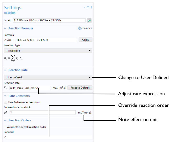
Figure 4-2: The reaction order can be manually specified for a user defined reaction rate.
