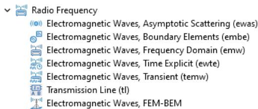
Figure 9: The Radio Frequency (RF) physics interfaces as displayed in the Model Wizard.
