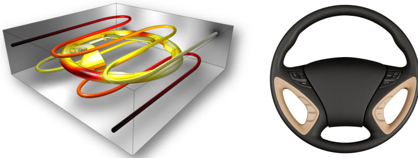
Figure 5: The heat transfer to the cooling channels embedded in a cooling mold is simulated to understand the controlled cooling of a polyurethane steering wheel. The Nonisothermal Pipe Flow interface is used in the model.
