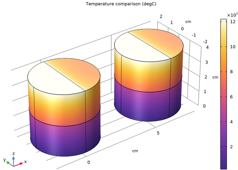
Figure 3: Temperature distribution with 3D model (left) and lumped model (right).
