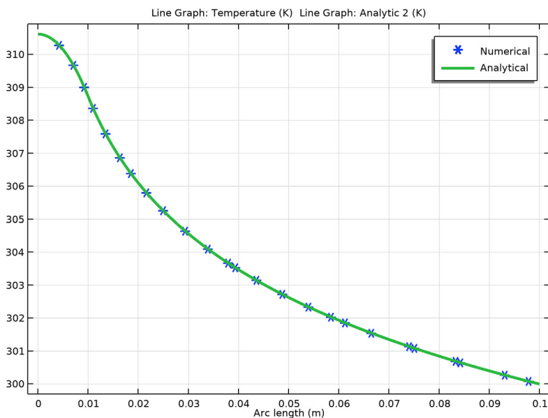
Figure 9: Comparison of the temperature obtained by COMSOL Multiphysics and an analytical solution (green line).
