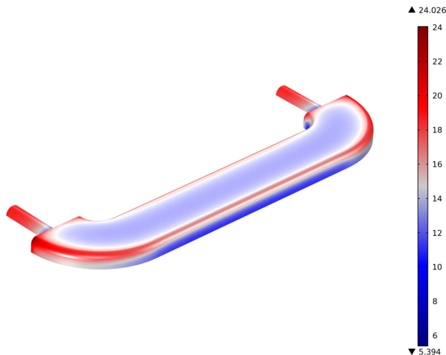
Figure 1: Thickness of the decorative deposited layer in a furniture fitting modeled using simulations based on secondary current distribution.
