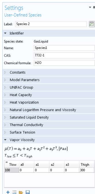
Figure 10-35: The Settings window for a User-Defined Species.
