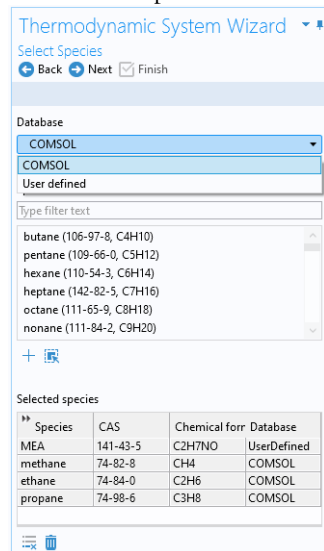
Figure 10-4: Thermodynamic System Wizard: Select Species.
