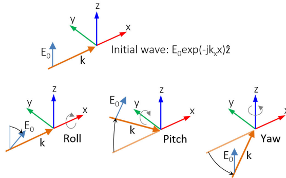
Figure 4-8: Schematic of the directions for the wave vector \mathbf{k} , the electric field \mathbf{E}_0 , and the roll, pitch and yaw rotations. The top image represents an initial wave propagating in the x direction with a polarization along the z direction.
