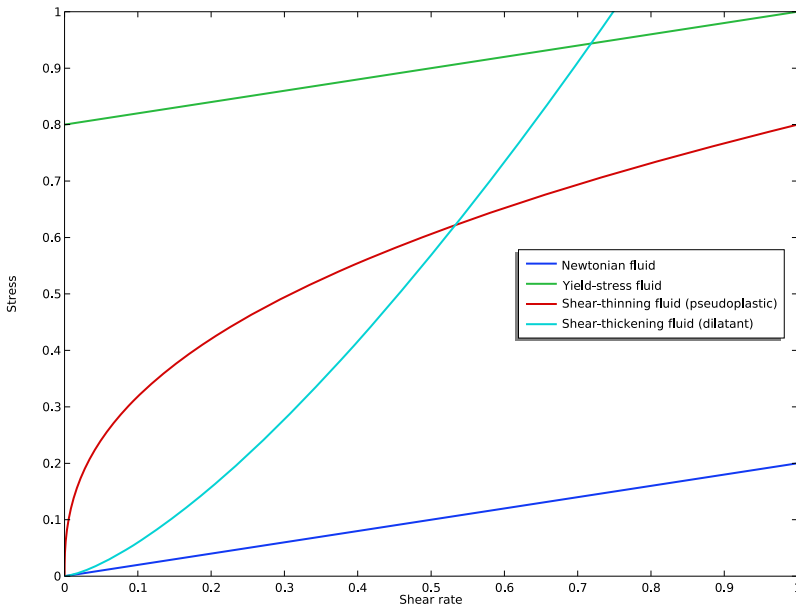
Figure 2: Conceptual behavior of shear stress versus shear rate for Newtonian, yield-stress, shear-thinning, and shear-thickening fluids.
