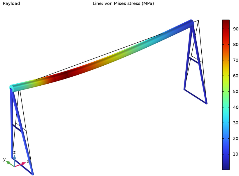
Figure 4: Equivalent stress caused by payload.
