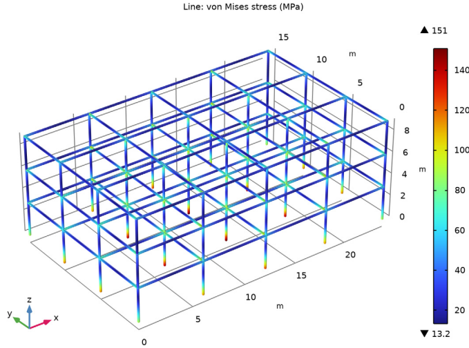
Figure 10: von Mises stress with CQC solution.
