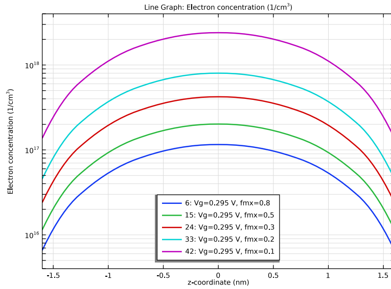
Figure 3: Electron concentration profile along the transverse centerline.
