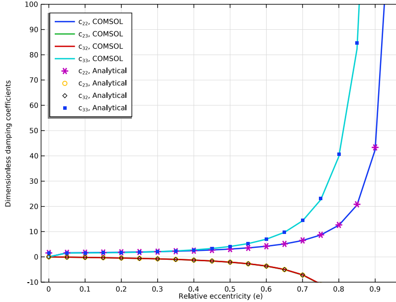
Figure 1: Damping coefficients.
