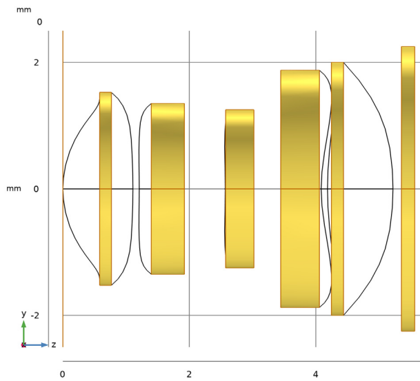
Figure 5: The Compact Camera Module obstruction cumulative selection.
