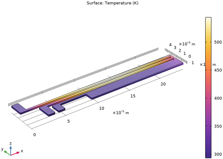
Figure 5: Temperature plot.
